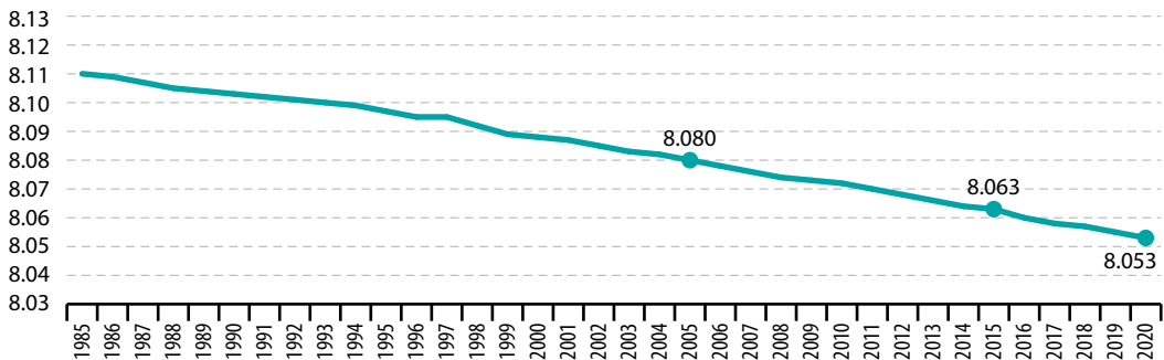
Figure 14.5: Global mean surface seawater acidity, 1985–2020 (pH value)
